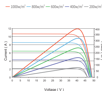
Current-Voltage &amp; Power-Voltage Curves (400W)
